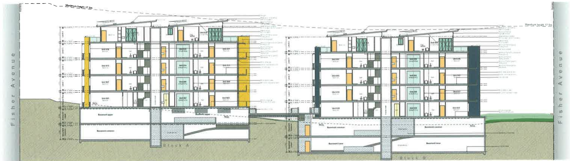
This architectural section drawing illustrates a multi-story building, likely a residential or institutional structure, with a maximum height of 17.5m. The drawing is oriented with Fisher Avenue to the left. The building is divided into two main sections, Block A and Block B, which are separated by a central vertical axis. Block A is a four-story structure with a central core and two wings. Block B is a taller, six-story structure with a similar layout. The drawing shows the internal layout, including rooms, corridors, and structural elements like walls, floors, and columns. Detailed annotations are provided for various components, such as walls, floors, and structural elements. The drawing is a technical representation of a building's internal structure and layout.
